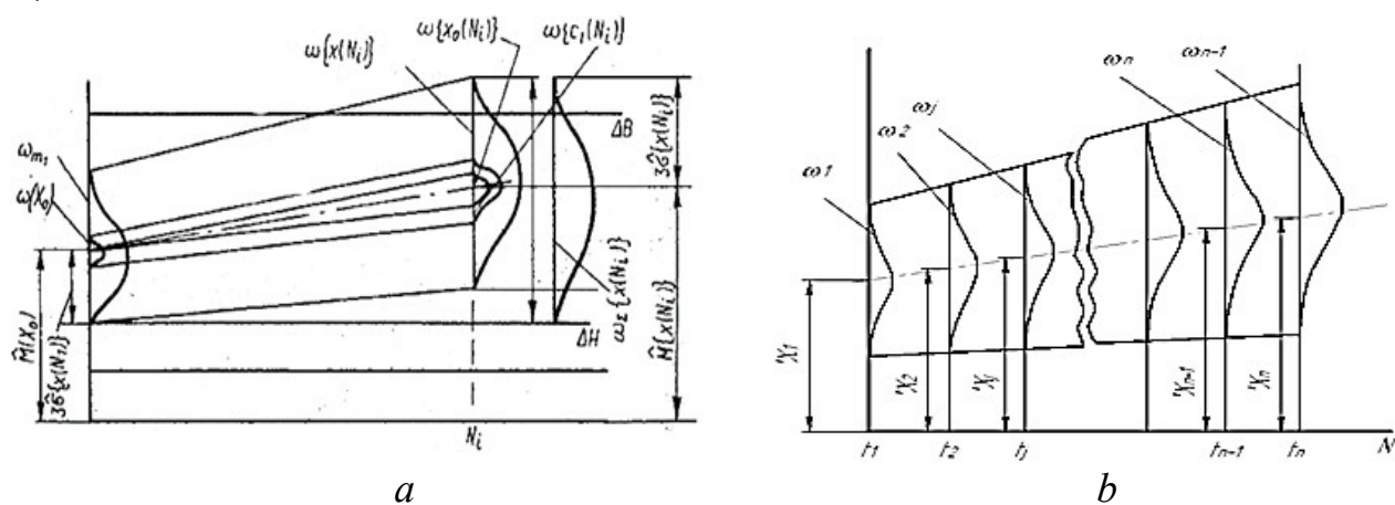
Fig. 1. Modeling of changes in the machining accuracy of a batch of blanks:
