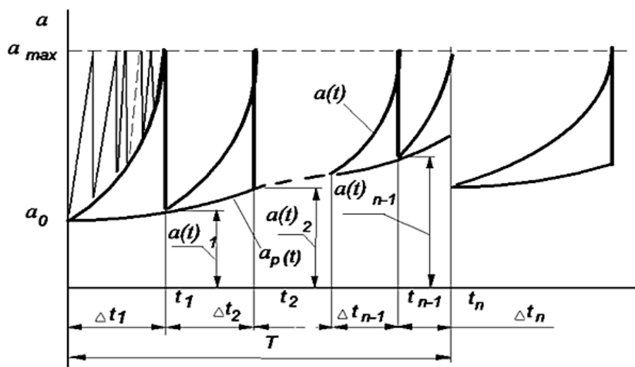
Fig. 3. Model of the technological service life of the machine according to V.V. Amalytsky [12]
