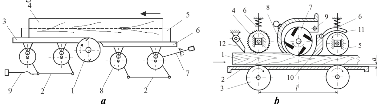
Fig. 1. Schematic diagrams of jointing and thickening machines: a – jointing machine; b – thickening machine
