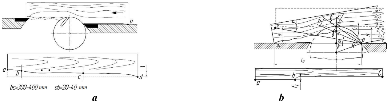
Fig. 3. Diagrams of machining errors depending on the placement of the locating surface of the rear table: a - tangential to the circle of the knife blades; b - below the circle of the knife blades
