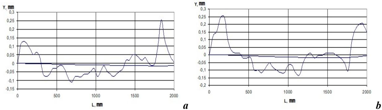
Fig. 5. Graphs of the distribution of the magnitude of errors of the machined surfaces along the length of the part:
