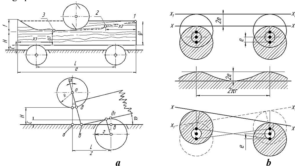
Fig. 4. Diagrams of errors of movable locating on a plate with rollers : a - locating on a plate with rollers; b - radial runout of the rollers
